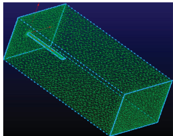
Figure 1: Complete 3-D unstructured wing grid created using Pointwise
