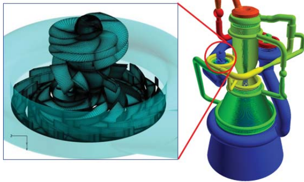
Figure 1: Pump side model of liquid oxygen turbo pump. Image provided by JAXA.
