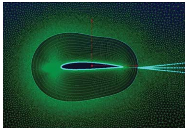
Figure 4: Close-up of 2-D hybrid airfoil grid created using Pointwise
