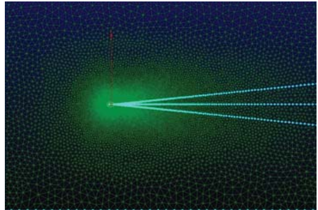
Figure 3: 2-D viscous airfoil grid (hybrid) created using Pointwise
